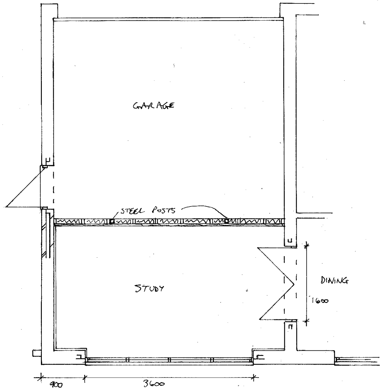
PROPOSED PLAN 1:50
