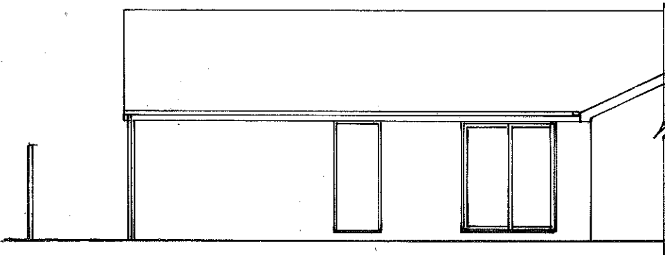
EXISTING REAR 1:100
